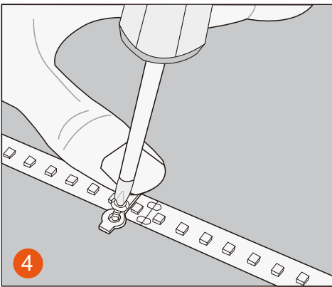
Use cross point electric screwdriver to install the screw. Repeat the steps 2-4 for next length installing.
