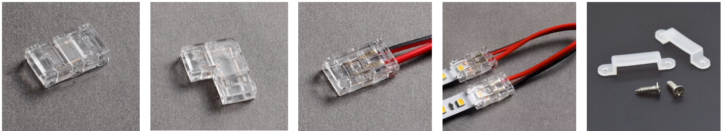
Strip to Strip ClipsL-Shape ClipsStrip to Wire ClipsStrip to Wire to Strip ClipsSilicone Mounting Clips
